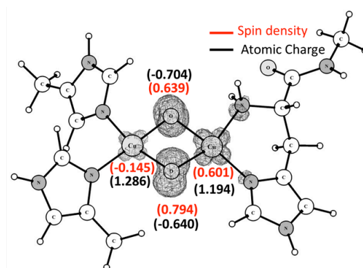
(b) Bis- \mu -oxo-Cu 2 (III) - Triplet
