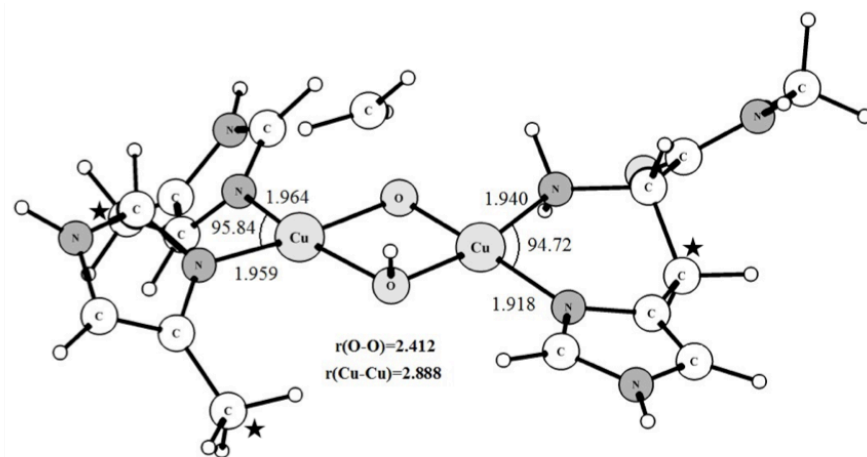
5(a) – Intermediate – 3 A
