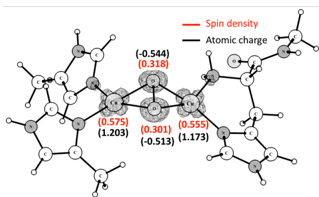
(a) peroxo-Cu 2 (II) - Triplet
