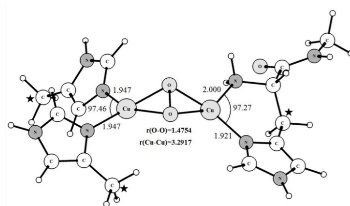
3(b) – Peroxo -3A
