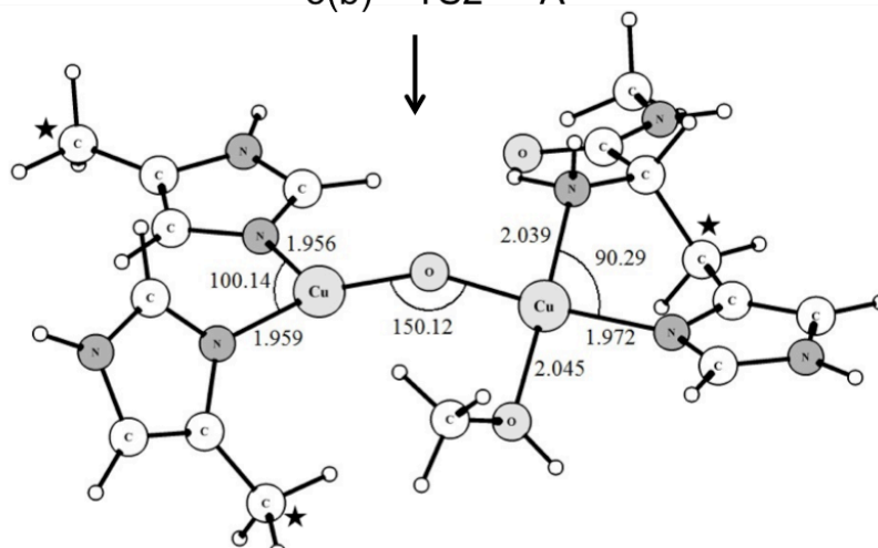
5(c) – Methanol Complex – 3 A
