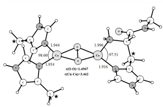
3(a) – Peroxo -1A
