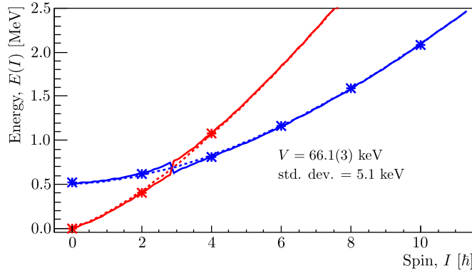
Figure 10. Variable moment of inertia (VMI) fits of the normal (red) and intruder (blue) bands in ^{186}\text{Hg} , performed in [34]. The dashed lines show the pure behavior of the bands, while the solid lines include a spin independent mixing parameter, V , to which the experimentally observed levels (crosses) are fitted. Here, a priori assignments of the experimental levels to each band is required and various assumptions were tested. The crossing of the bands can be seen around I = 3 , indicating that the 4_1^+ state is predominantly of the intruder configuration.
