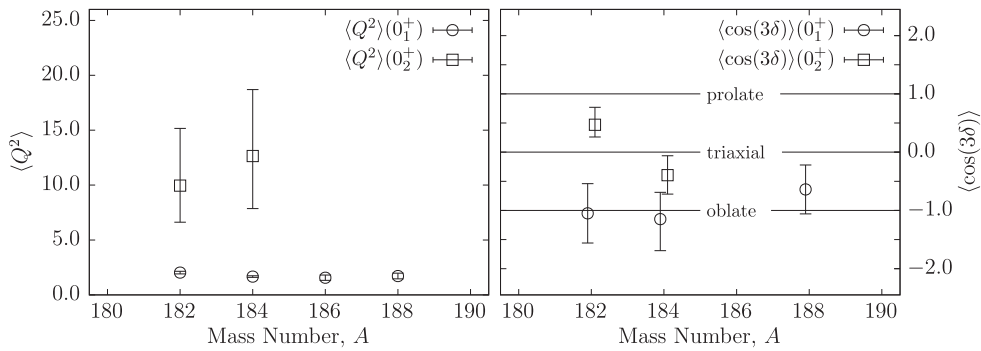
Figure 8. The \langle Q^2 \rangle and \langle \cos(3\delta) \rangle values representing the overall deformation and the axial asymmetry, respectively of the 0_1^+ (open circles) and 0_2^+ (open squares) states in ^{182-188}\text{Hg} . These were extracted from the matrix elements obtained in [53].
