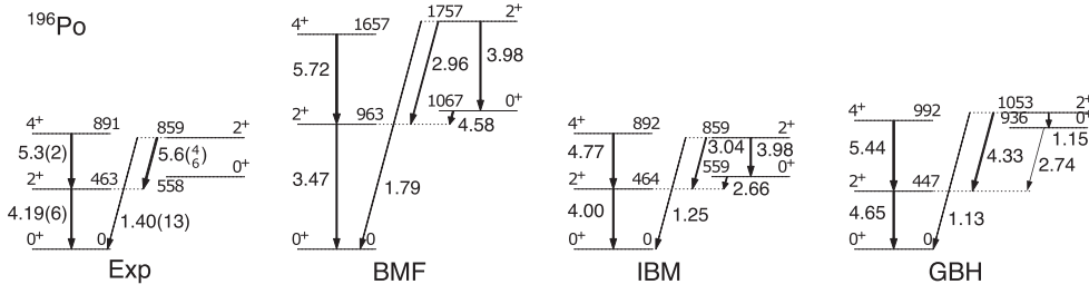
Figure 11. Experimental level scheme and Q_t values in ^{196}\text{Po} compared to the predictions of calculations performed within the beyond-mean-field (BMF) [47], interaction-Boson (IBM) and general-Bohr-Hamiltonian (GBH) models. Adapted from [57] under a CC BY 3.0 licence.
