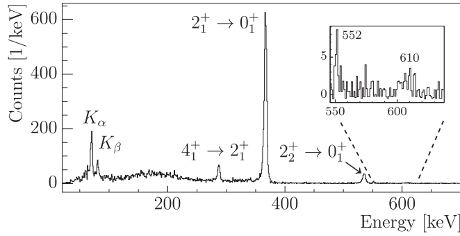
Figure 3. \gamma -ray energy spectrum following the Coulomb-excitation of ^{184}\text{Hg} induced by a ^{120}\text{Sn} target, Doppler-corrected for transitions in ^{184}\text{Hg} . The population of the yrast and non-yrast states in ^{184}\text{Hg} as well as intense mercury K -shell x-ray peaks are observed. The inset shows part of the spectrum where a weak 4_2^+ \rightarrow 2_2^+ \gamma -ray peak (552 keV) and ( 2_3^+ \rightarrow 0_2^+ and 2_3^+ \rightarrow 2_1^+ ) doublet (around 610 keV) in ^{184}\text{Hg} are visible.
