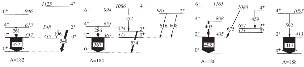
Figure 4. Part of the low-energy level schemes of the even-even ^{182-188}\text{Hg} isotopes. Widths of the arrows are proportional to the observed \gamma -ray intensities normalized to the 2_1^+ \rightarrow 0_1^+ transition. Energies of \gamma -ray transitions and levels (italics) are given in keV. Adapted from [53].
