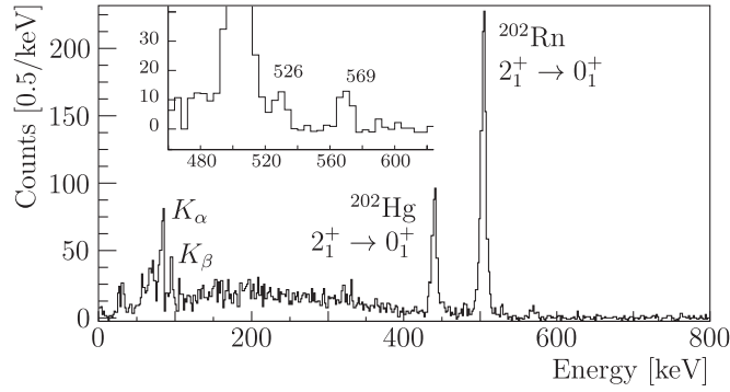
Figure 6. \gamma -ray energy spectrum following the Coulomb excitation of ^{202}\text{Rn} induced by a ^{120}\text{Sn} target, Doppler-corrected for transitions in ^{202}\text{Rn} . The first-excited 2^+ state in ^{202}\text{Rn} is populated and, more weakly, the 2_2^+ and 4_1^+ states (inset shows the 526 keV 2_2^+ \rightarrow 2_1^+ and 569 keV 4_1^+ \rightarrow 2_1^+ transitions with a 4 keV bin width). Additionally, an excess of K -shell x-rays is observed, just as in the Hg, Pb and Po cases. Isobaric contamination was present in the beam from the stable ^{202}\text{Hg} , which is also excited and can be observed in the \gamma -ray spectrum. Adapted from [58] under a CC BY 3.0 licence.
