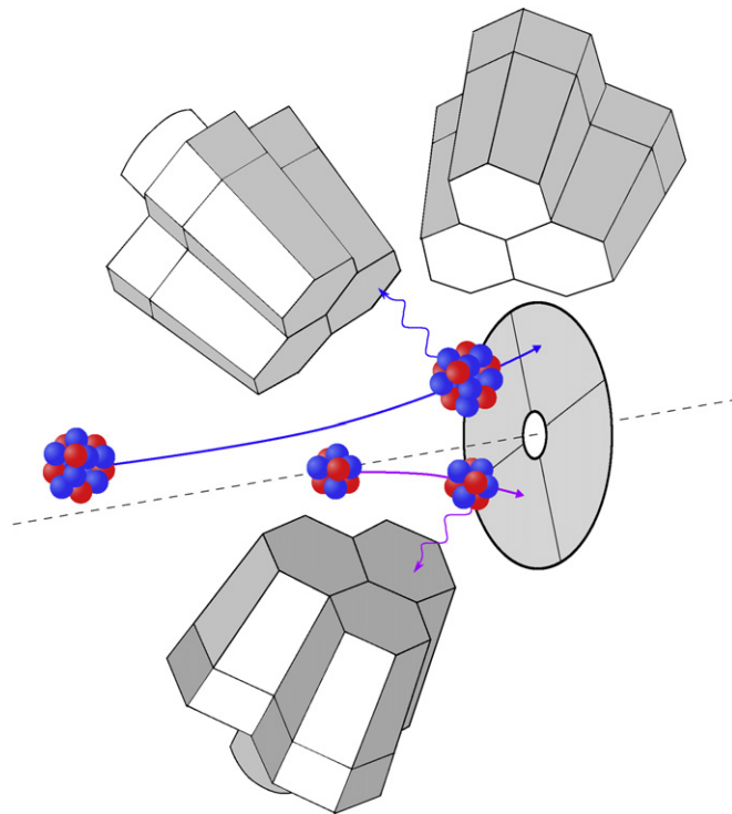
Figure 2. A schematic representation of the Coulomb-excitation experiments performed with Miniball at REX-ISOLDE in this campaign. A heavy radioactive ion is impinged on lighter target species and both the scattered projectile and recoiling target nucleus are forward focused in the laboratory frame of reference. This allows coincident detection of both scattering partners in the DSSSD detector of Miniball, along with the de-excitation \gamma -rays that follow inelastic events.
