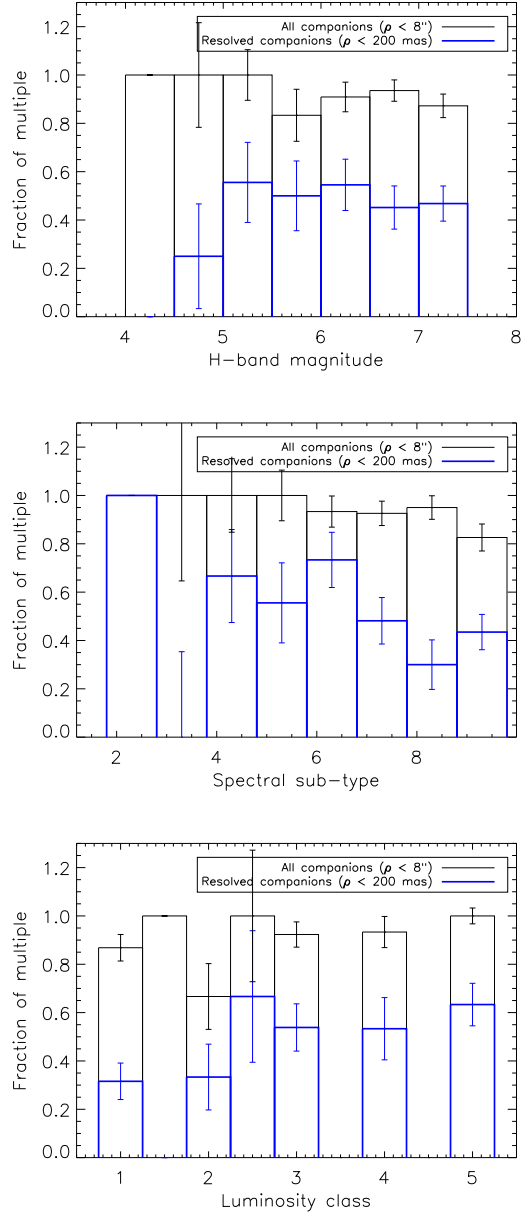
Fig. 14.— Fraction of multiple systems as a function of their H -band magnitude ( top panel ), of their spectral sub-type ( middle panel ) and of their luminosity class ( bottom panel ).
