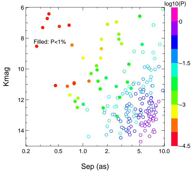
Fig. 8.— Probability P_{\text{spur}} for the companions detected in the NACO FOV to result from chance alignment. The probability P_{\text{spur}} is color-coded in the K s-band magnitude vs. angular separation plane. Filled symbols indicate P_{\text{spur}} < 0.01 while open symbols are used for P_{\text{spur}} \geq 0.01 .
