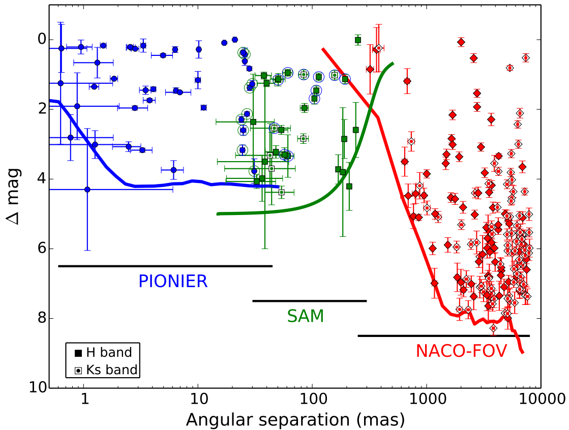
Fig. 7.— Plot of the magnitude difference ( \Delta \text{mag} ) vs. angular separations ( \rho ) for the detected pairs. Only one detection per object has been considered, and the H -band has been preferred whenever available. The solid lines indicate the median H -band sensitivity of our survey across the different separation ranges. The Ks sensitivity curves are similar. Different colors indicate observations with different instrumental configurations (PIONIER: blue, NACO/SAM: green, NACO FOV: red) while different symbols indicate different observational bands ( H : filled, Ks : open). Large circles indicate objects detected by both SAM and PIONIER.
