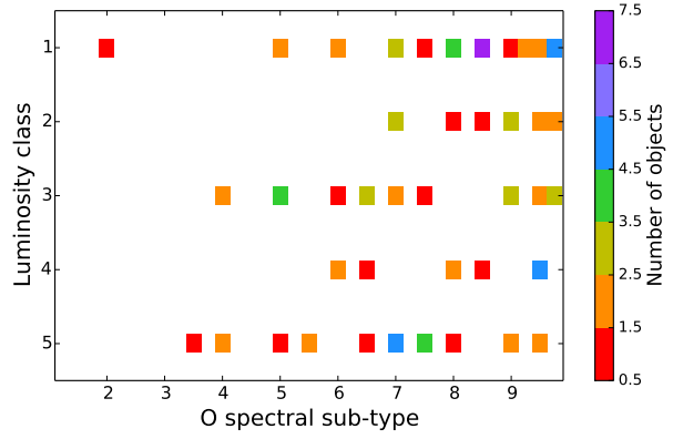
Fig. 2.— Distributions of luminosity classes vs. spectral sub-types of SMASH+ targets in our main sample.
