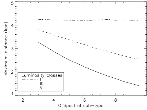
Fig. 3.— Maximum distance of a single star for its H -band apparent magnitude to be brighter than the SMASH+ cutoff magnitude ( H = 7.5 ) as a function of spectral sub-type and luminosity class. The figure ignores the effects of extinction and multiplicity, which act in opposite directions.
