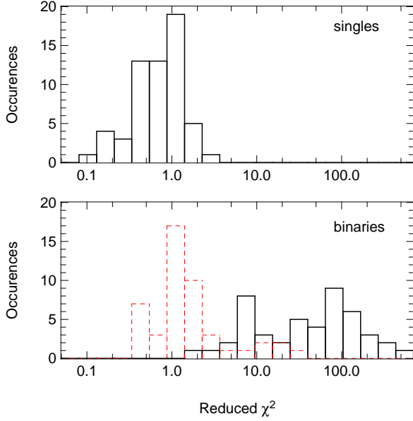
Fig. 4.— Distribution of the PIONIER reduced \chi^2 obtained with the single-star model (Eq. 5; solid line) for the unresolved targets ( upper panel ) and the resolved pairs ( lower panel ). The dashed line gives the distribution of the reduced \chi^2 obtained with the best-fit binary model.
