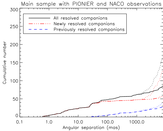
Fig. 10.— Same as Fig. 9 but restricted to the 96 targets from our main sample that have been observed both with PIONIER and NACO.
