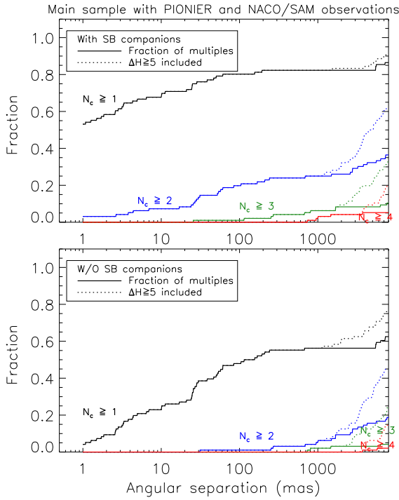
Fig. 13.— Cumulative fraction of multiple systems for a minimum number of companions of 1, 2, 3 and 4. The top panel includes the unresolved spectroscopic and eclipsing companions whereas the bottom panel does not.
