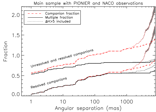
Fig. 12.— Cumulative fraction of multiple systems (solid line) and average fraction of companions per star (dashed-dotted lines) for increasing angular separations. The upper curves account for the spectroscopic and eclipsing companions whereas the bottom ones do not. Shaded gray areas indicate the statistical contribution of spurious detections due to chance alignment.
