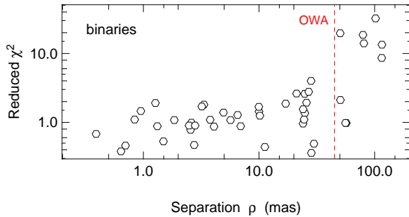
Fig. 5.— Reduced \chi^2 plotted against the separation for the best-fit binary models. Poor fits are only observed outside the outer working angle (OWA).
