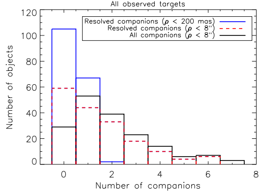
Fig. 11.— Histogram of the number of companions per target for the full separation range and for separations below 200 mas. All companions account for resolved companions within 8'' as well as for known spectroscopic and eclipsing companions.
