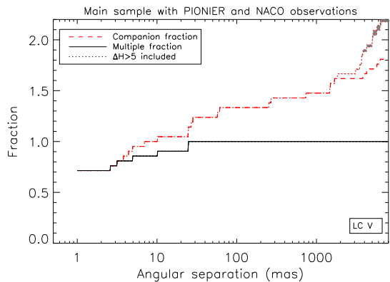
Fig. 15.— Break down of Fig. 12 for luminosity classes I, III and V. The curves include the unresolved E/SB companions.
