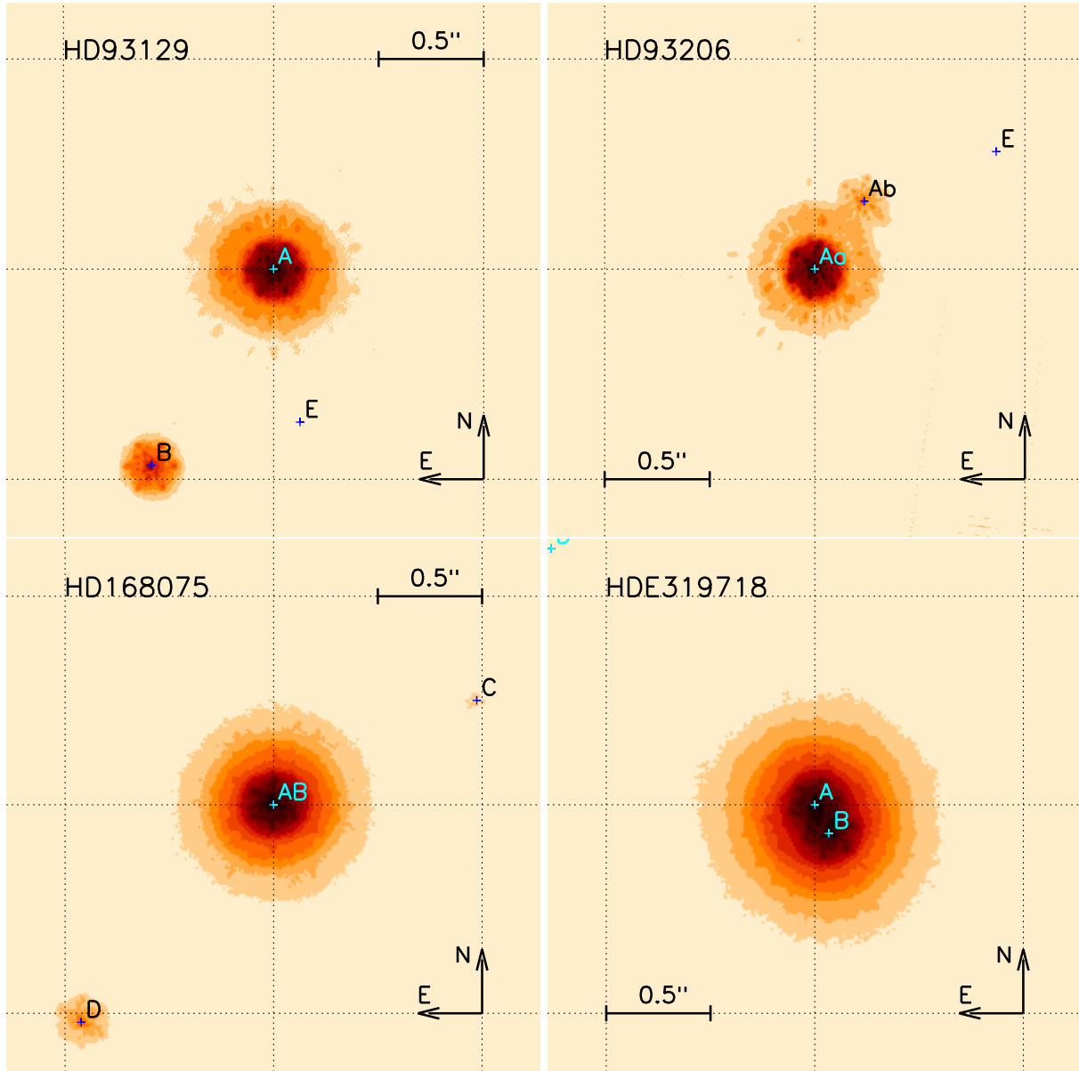
Fig. 6.— Examples of NACO data sets featuring the multiple systems HD 93129, HD 93206, HD 168075 and HD 319718. Only the central 2'' of the NACO FOV are shown. The faint E components of HD 93129 and HD 93206 are not visible with the adopted cut but their positions are marked.
