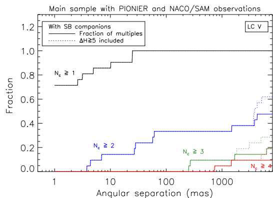
Fig. 16.— Break down of Fig. 13 for luminosity classes I, III and V. The curves include the unresolved E/SB companions.
