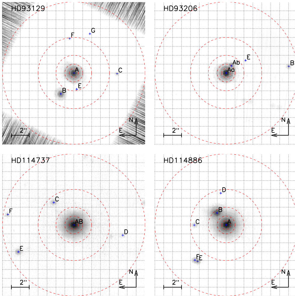
Fig. 17.— NACO images of the surroundings of HD 93129, HD 93206, HD 114737 and HD 114886. Dotted lines are separated by 1'' . Dashed circles have radii of 0.5'' , 1'' , 2'' , 4'' and 8'' . Companions are identified by a letter and their position in the field is marked by a cross-hair (+).
