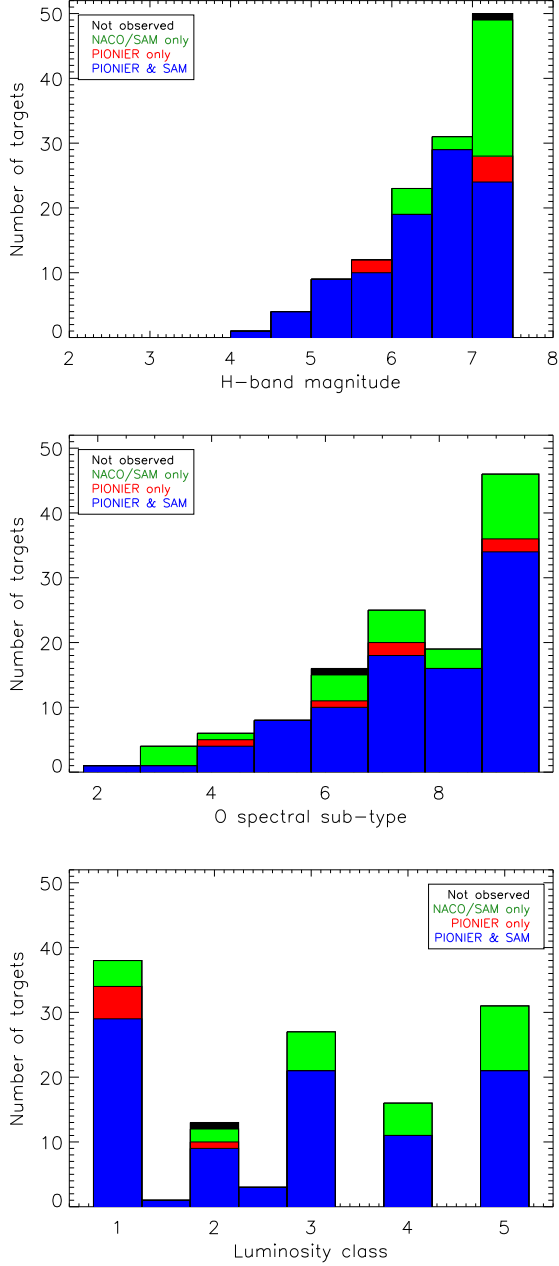
Fig. 1.— Distributions of H -band magnitudes ( upper panel ), spectral sub-types ( middle panel ) and luminosity classes ( lower panel ) of SMASH+ targets in our main sample. Fractional luminosity classes indicate uncertain classification between the two neighboring classes.
