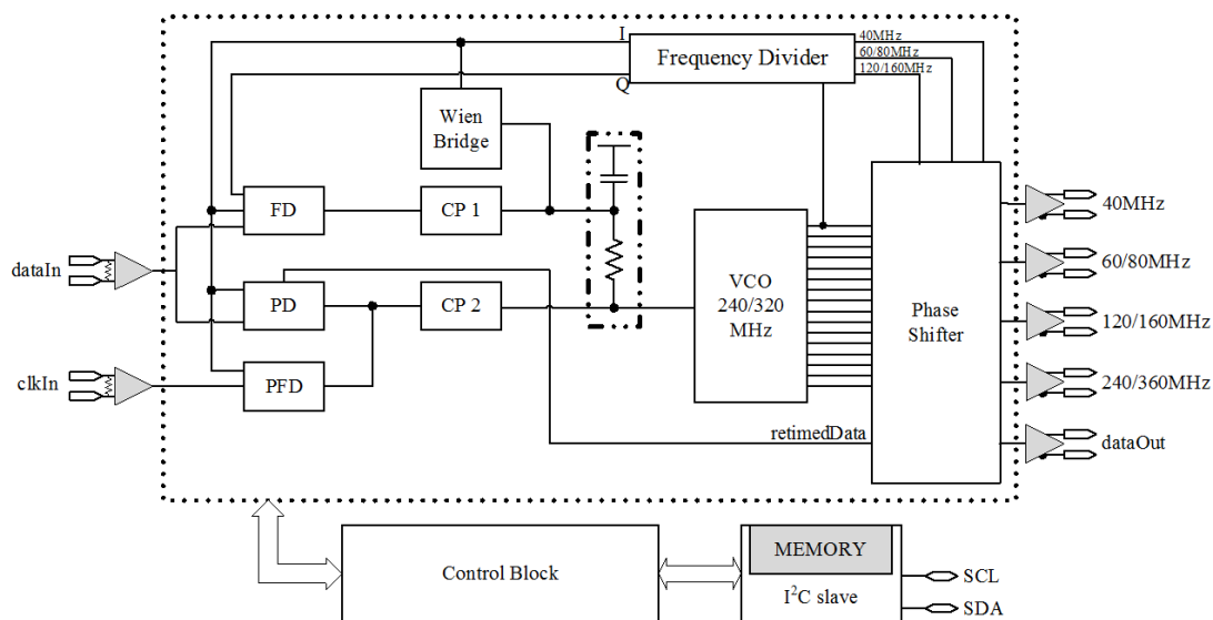
Figure 1. eCDR-PLL ASIC simplified block diagram.
