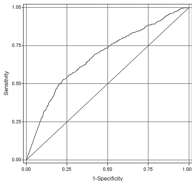
Figure 2 Receiver operating characteristic curve analysis showing the infliximab threshold that best discriminated disease activity, as measured by C-reactive protein (concentration \leq 5 mg/L was defined as inactive disease).
