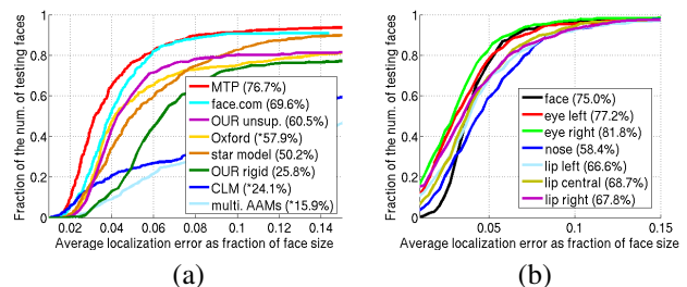
Figure 6. Cumulative error distribution for facial point localization on AFW. (a) Comparison with other methods. (b) Cumulative error for each facial landmark.
