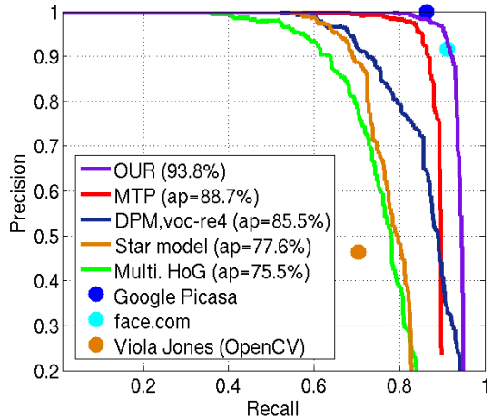
Figure 3. Precision-recall curves for AFW. With only 900 training images our method outperforms most of the other methods. Note that this evaluation is done on all the test faces of AFW.
