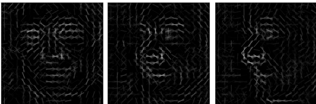
Figure 5. Mixtures obtained without pose estimation. Even without knowing the pose of the faces at training time we are able to learn meaningful models.
