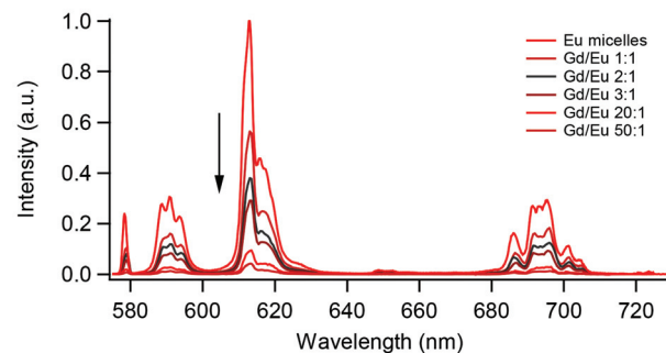
Fig. 6 Corrected and normalized luminescence spectra of micelles consisting of Gd/Eu-DTPA-BC 12 PheA (top) and Gd/Eu-DTPA-BC 14 PheA (bottom) (H 2 O, 10 -4 M, λ exc = 290 nm, 298 K).
