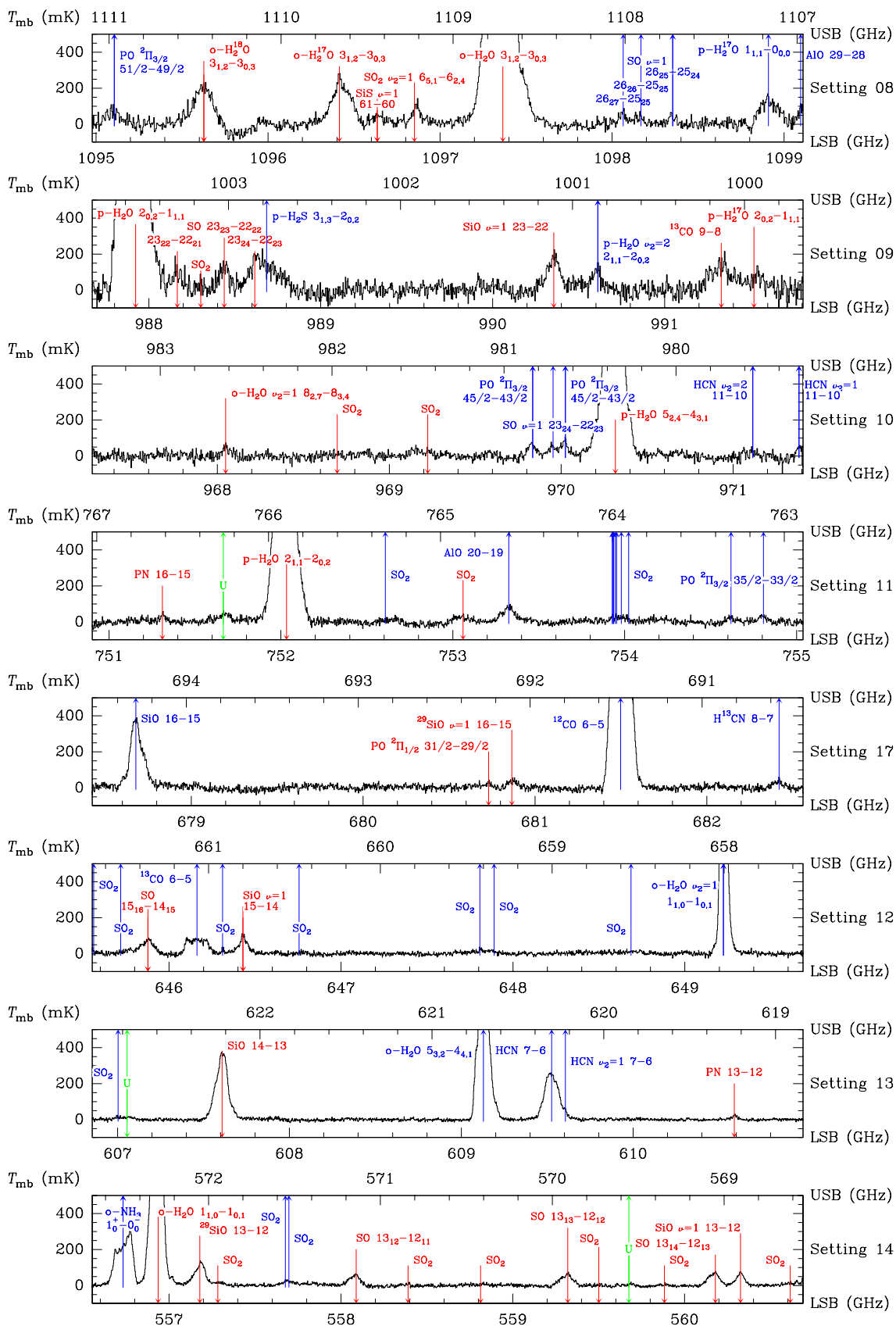
Fig. B.1. Full WBS bandwidth HIFI results for VY CMa for LO frequencies of 1102.9 GHz and lower. Quantum numbers for SO 2 transitions are not given for clarity.
