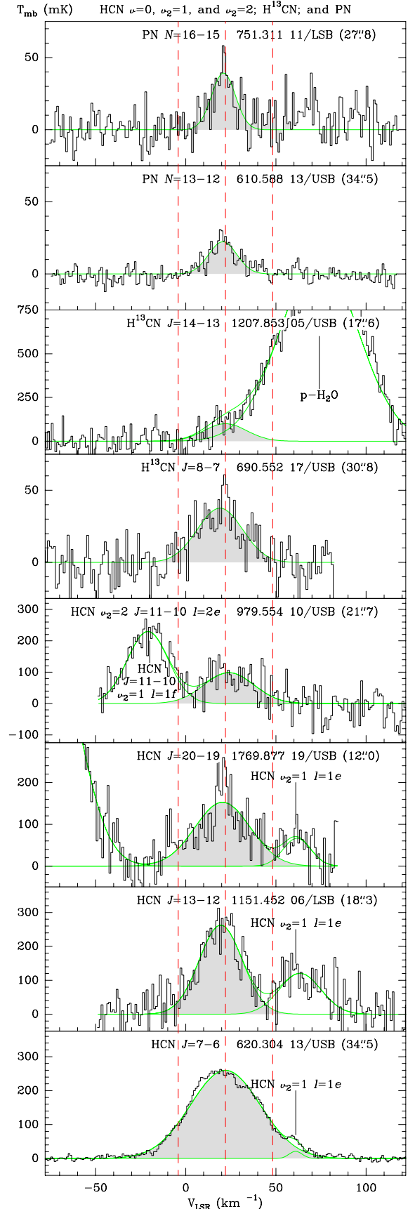
Fig. A.5. Same as Fig. 3 for the detected lines of HCN, \text{H}^{13}\text{CN} , and PN.
