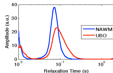
Fig.2 UBO sites show an increased peak width and gmT2 in the T2-distribution
