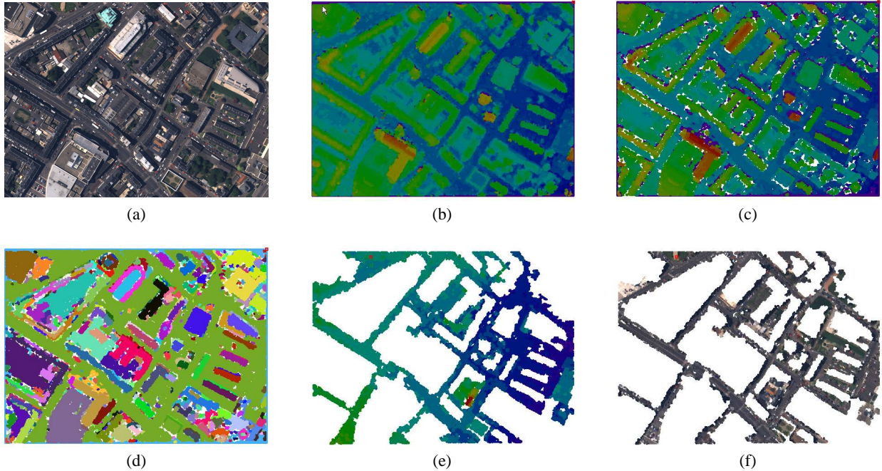
Figure 3: Results of ground level extraction for a sub-area of the airborne laser DEM of the Amiens region. (a) Part of an aerial image showing the sub-area of the Amiens region. (b) Part of the original DEM with altitude coloring. (c) The DEM part after smoothing and isolated point removal. (d) The result of automatic segmentation. (e) The automatically extracted ground level. (f) The extracted ground level with texture mapping for visual verification.
