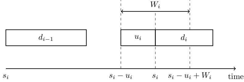
Figure 1: Illustration of a time window at customer i .
