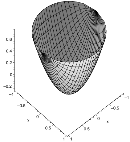
\mathcal{L}_2(z) for x^2 + y^2 \leq 1
