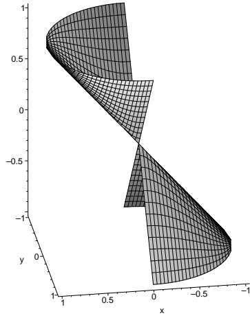
Fig. 1. \mathcal{L}_1(z) for x^2 + y^2 \leq 1
