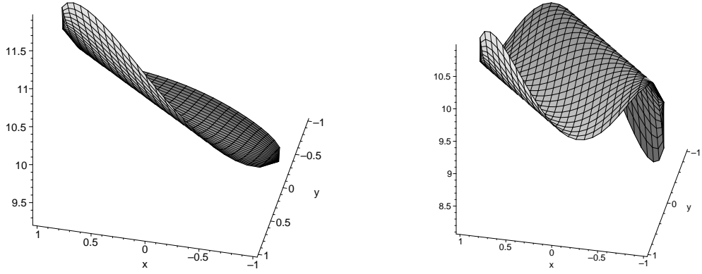
Fig. 2. \mathcal{P}(z) with (\lambda_1, \lambda_2) = (3/5, 4/5) \mathcal{P}(z) with (\lambda_1, \lambda_2) = (-\sqrt{2}/2, -\sqrt{2}/2)
