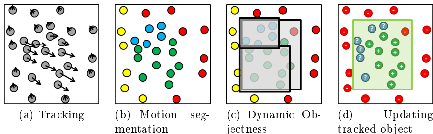
Fig. 3. The tracked feature points shown in (a) are grouped in (b) according to their motion. Our novel Dynamic Objectness allows to locate possible object regions (c). Using the propagated points, the tracked object region can robustly be updated (d).
