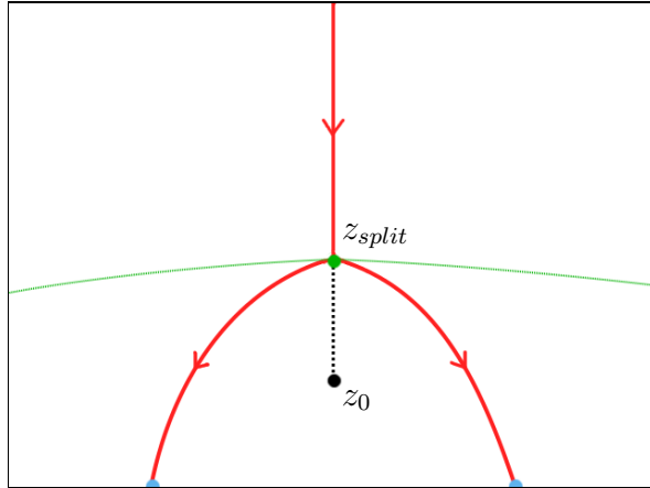
Figure 1: Schematic drawing of the split flow tree for our representative charge system. The flow coming in from the top (red line) reaches the wall of marginal stability (green line) at the splitpoint z_{split} (green) before it would reach the crash point z_0 (black). One also sees the single flows for each center starting from the split point until they reach the boundary of moduli space (blue).
