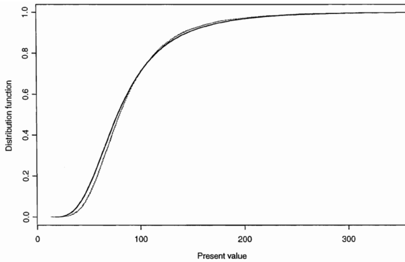
Figure 1: Distribution function of the upper bound A_{upp} (black) for \alpha_t = 10 ( t = \dots, 10 ), compared to a simulated version of the distribution of A (grey).
