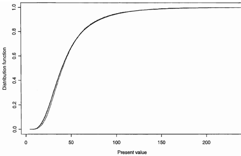
Figure 3: Distribution function of the upper bound A_{upper} (black) for \alpha_t = t ( t = \dots, 10 ), compared to a simulated version of the distribution of A (grey).
