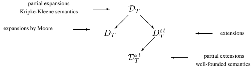
Figure 1.2 Operators and semantics associated with autoepistemic logic
