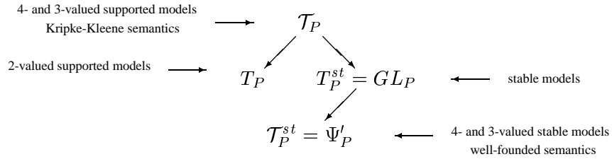
Figure 1.1 Operators and semantics associated with logic programming
